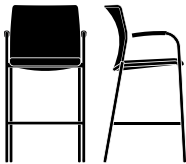
3815 Bar Stool with Arms W 22" D 22.5" H 42.5" SH 28.5" AH 35.75"
