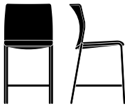
3811 Armless Counter Stool W 19.75" D 22.5" H 39" SH 25"
