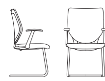
9331 Guest Chair, Upholstered With Arms or Armless - 9330 W 23.5" D 22" H 37.25" SH 18.5" AH 26.5"
