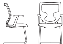
9341 Guest Chair, Mesh Back With Arms or Armless - 9340 W 23.5" D 22" H 37.25" SH 18.5" AH 26.5"
